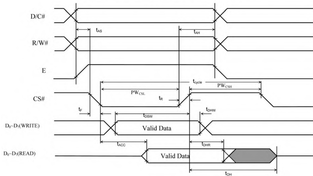
Figure 34 : 6800-series MCU Parallel Interface Characteristics
