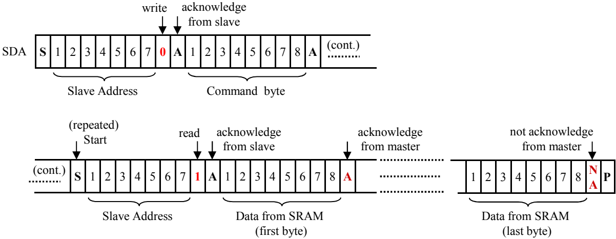
Figure 7. Read From SRAM
